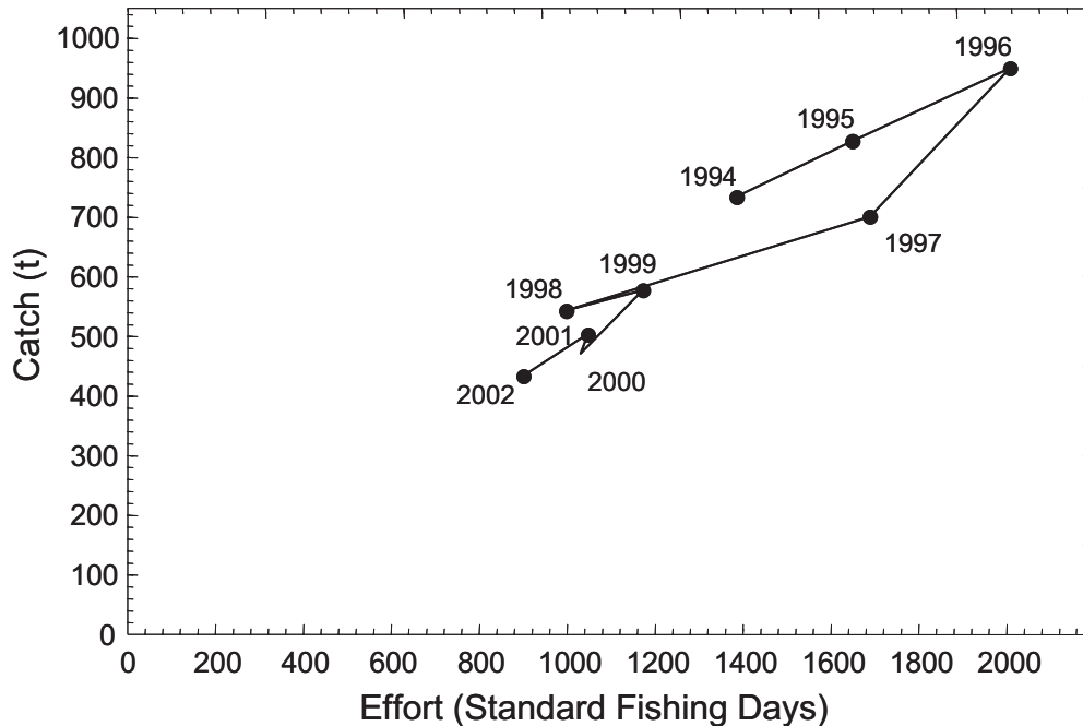
Figure 3 Relationship between total annual catch and total annual standardised trap fishing effort in the NDSMF in the period from 1994 to 2002.
