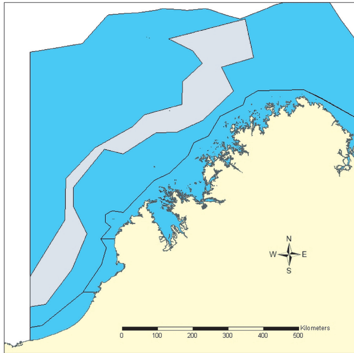
Figure 6 Spatial distribution of effort obtained from the VMS database for all vessels from 1999 to 2002 is depicted in light grey (area of the NDSMF in light blue).
