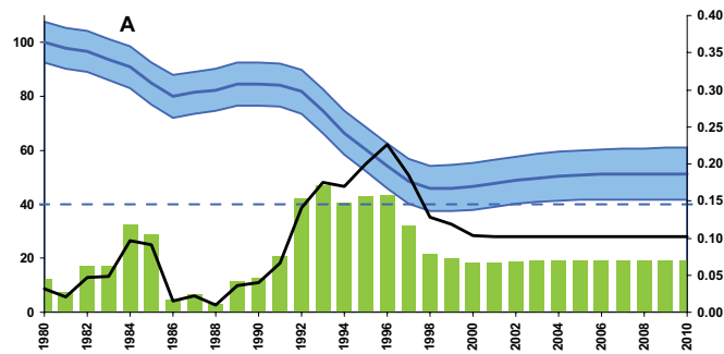
Figure 12 Red emperor spawning biomass (with 95% confidence intervals) (blue), catch ÷ 5 (green) both with scale on left axis, and fishing mortality (black) with scale on right axis for base case scenario, no efficiency increase, and effort=900 days after 2002.
