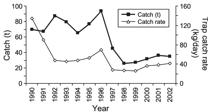
Figure 18 Annual total catch level and trap catch rate of spangled emperor in the NDSMF from 1990 to 2002.
