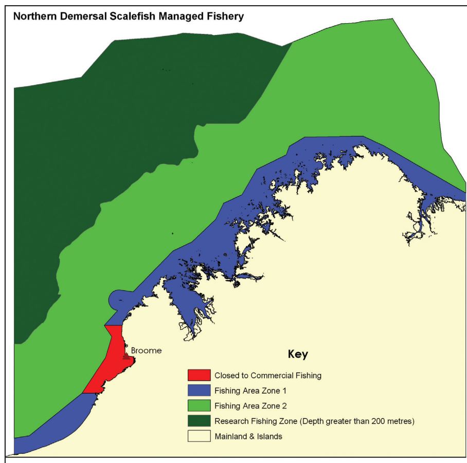
Figure 2 Location, boundaries and zones within the NDSMF in the Kimberley region of north-western Australia.
